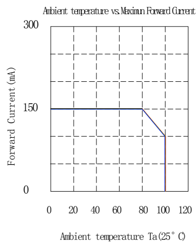
Derating
