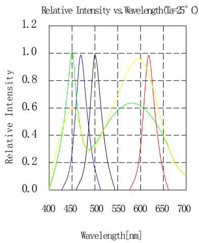
Spectral Distribution
