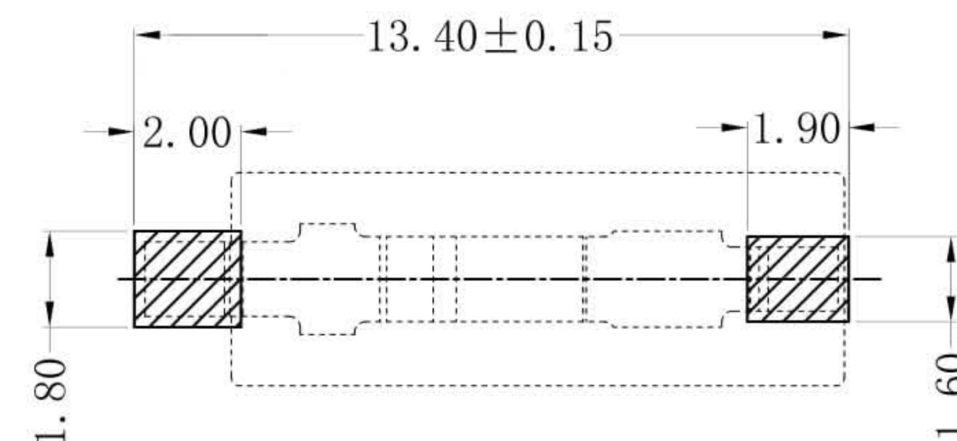
SUGGESTED PCB LAYOUT (COMPONENT SIDE)
